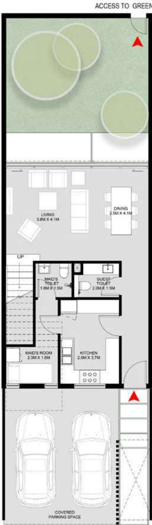
Ground Floor
